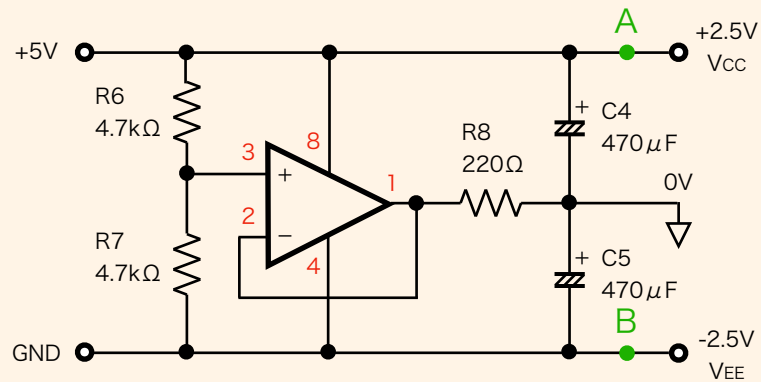
1/2 IC2 NJM2904D
