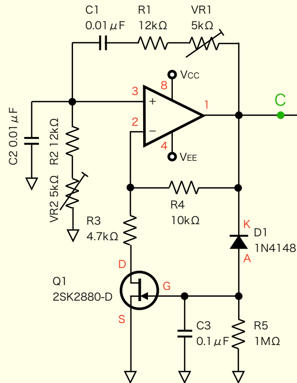
1/2 IC1 NJM4580DD
